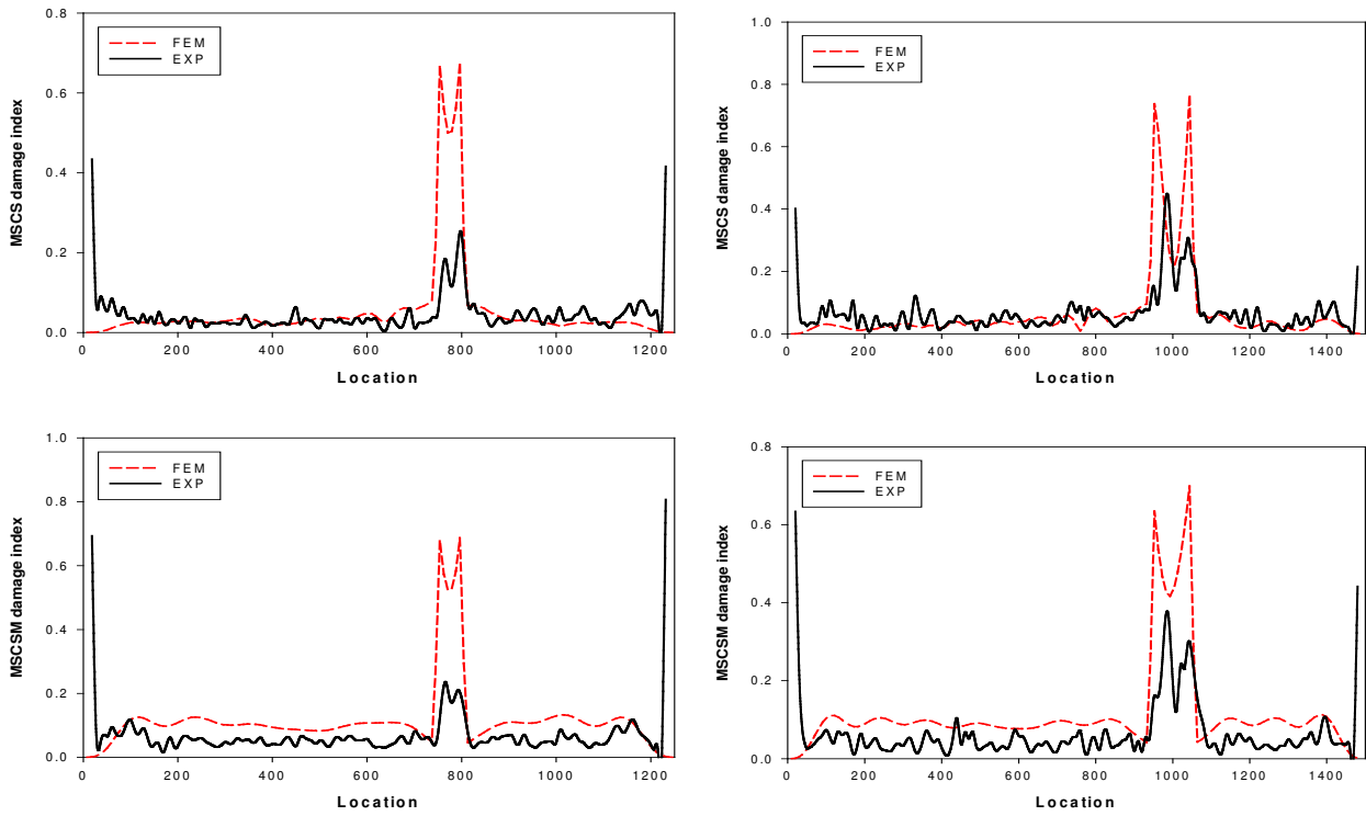
Fig 3. Damage detection methods for beams with FF boundary conditions; Beam 1 – left; Beam 2 – right
