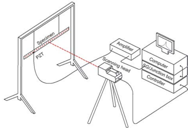
Fig 2. Scheme of experimental set-up
