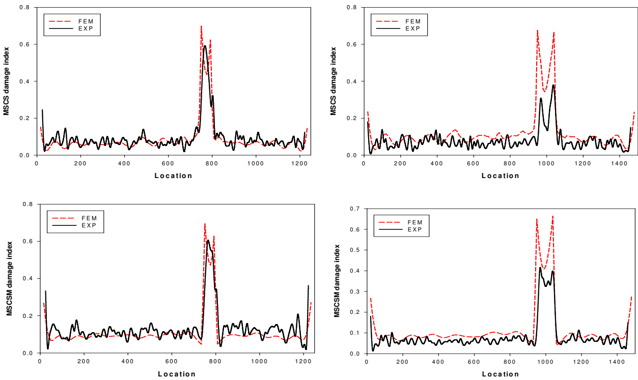
Fig 4. Damage detection methods for beams with CL boundary conditions; Beam 1 – left; Beam 2 – right
