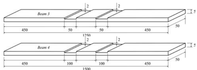
Fig 5. Geometry and dimensions of the test beams containing mill-cut damage at multiple locations
