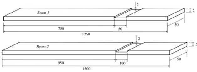
Fig 1. Geometry and dimensions of the test beams containing mill-cut damage at single location
