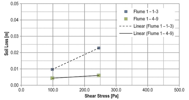
Fig. 13. Erosion rates flume 1 (unvegetated); soil loss and shear stress, steep trend line = high erosion rate, focus on the upper (“1-3”) and lower (“4-9”) flume parts, September 2014
