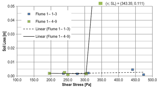
Fig. 10. Erosion rates flume 1 (vegetated); soil loss and shear stress, steep trend line = high erosion rate, focus on the upper (“1-3”) and lower (“4-9”) flume parts, September 2014
